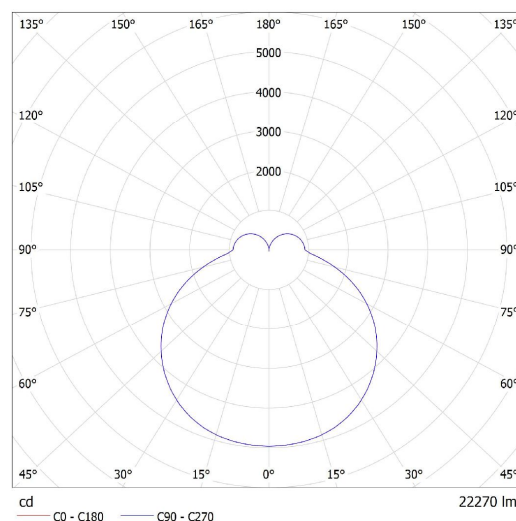
Lucis IR.L11.1200M.1 IZAR R MAX LED / LDC (Polar)
